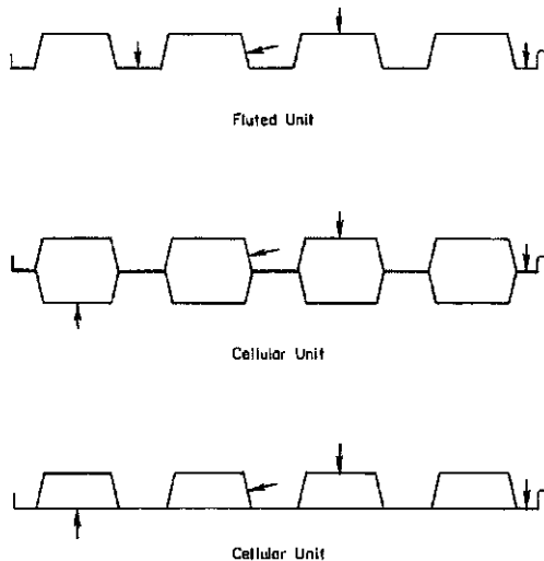
FIG. 3 Typical Location of Thermocouples
