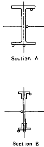
FIG. 2 Typical Thermocouple Distributions
