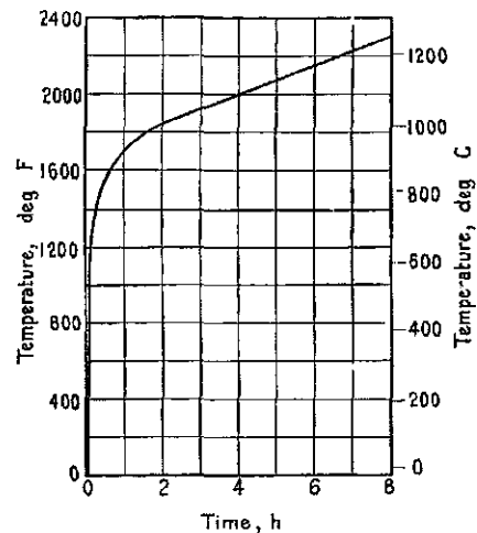
FIG. 1 Time-Temperature Curve
